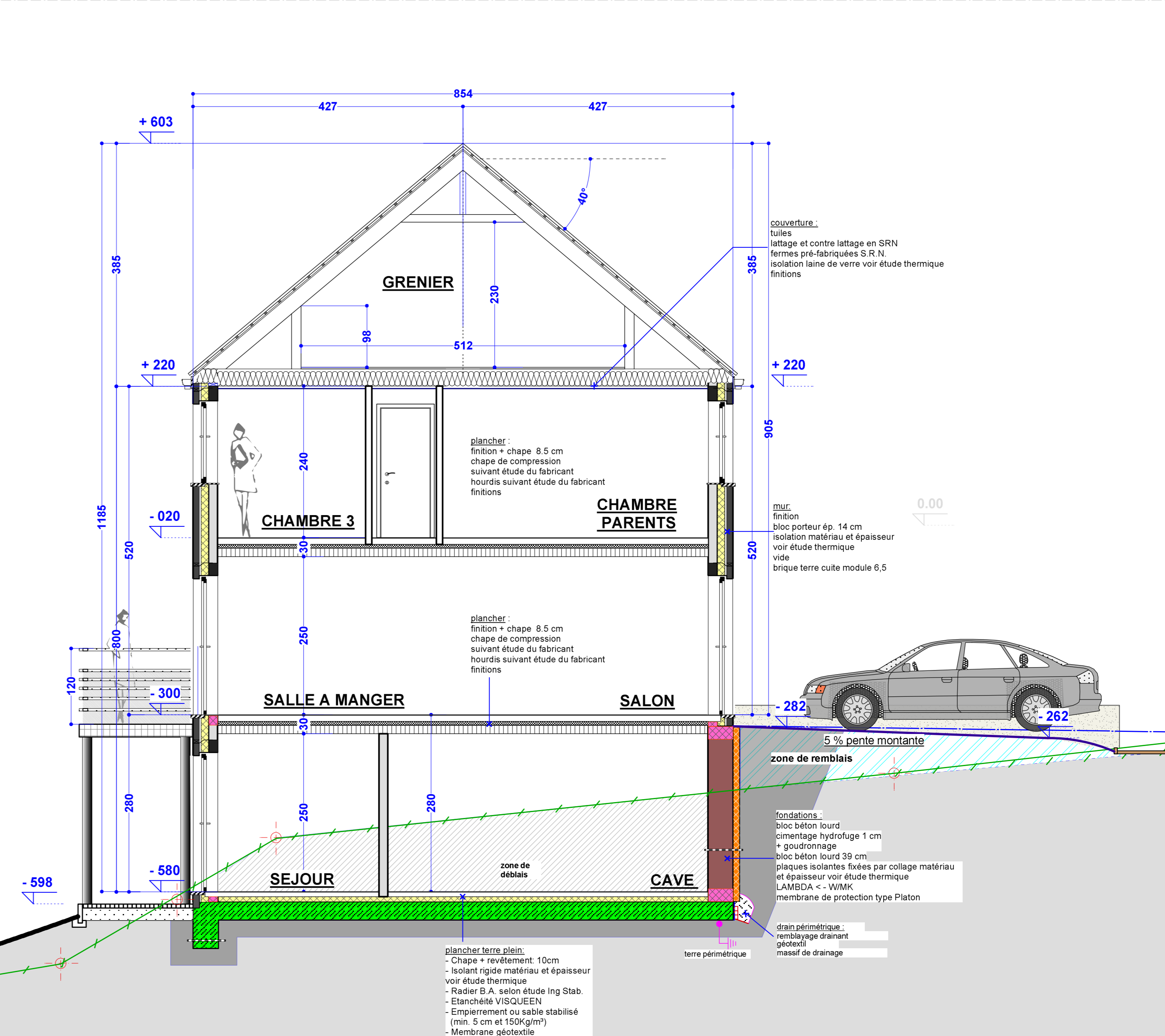
COUPE LOT 9 ECH 1/50
