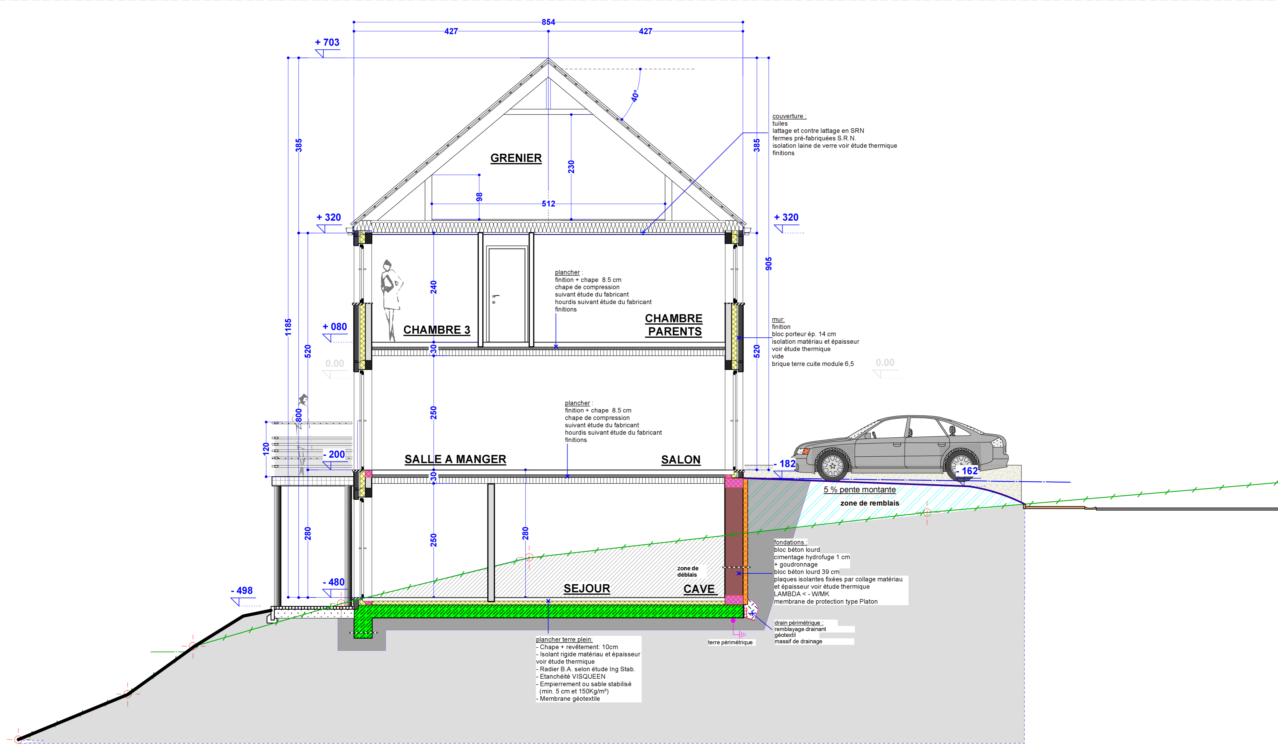
COUPE LOT 10 ECH 1/50
