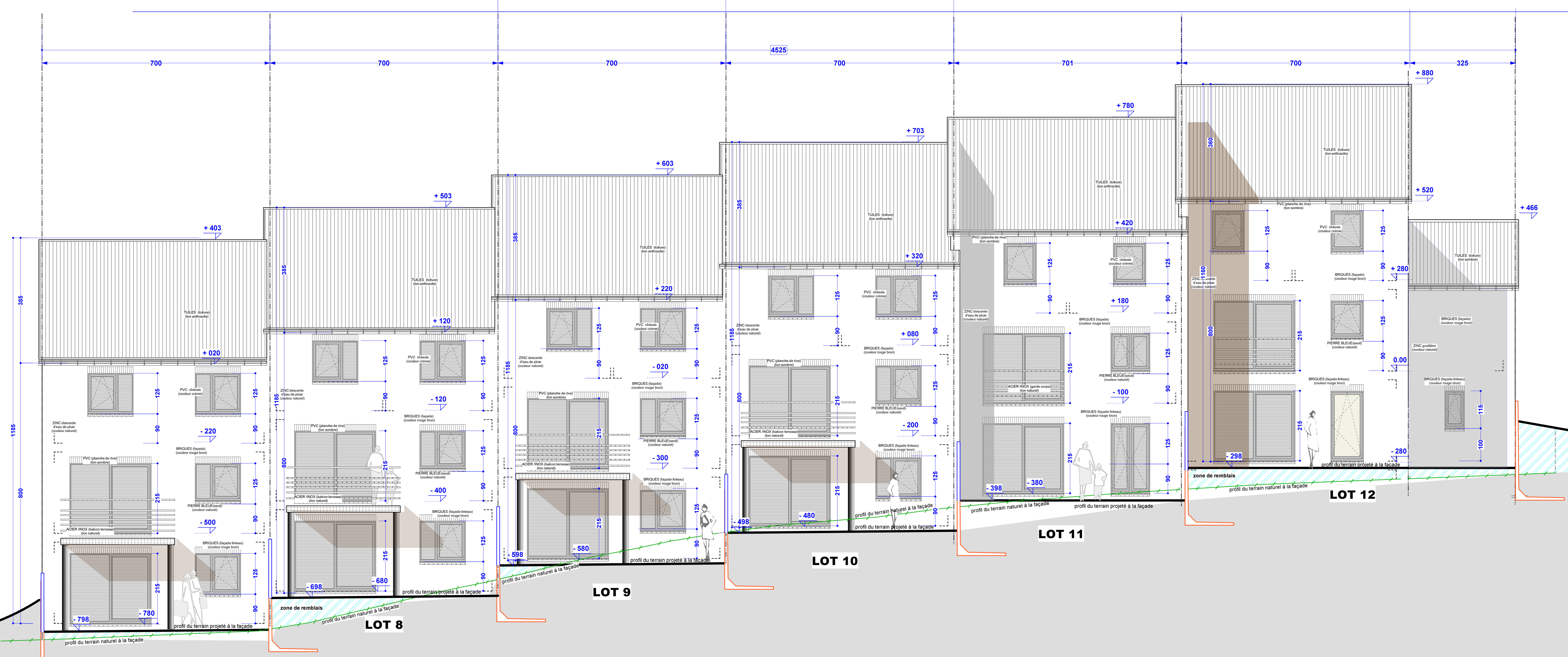
ELEVATION ARRIERE ECH 1/50
